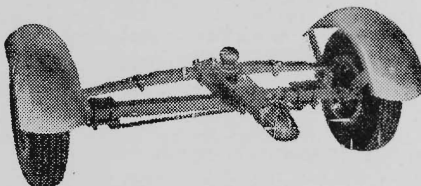
The Hendy balanced caravan dolly, counteracts pitch, roll and vibration. Takes 2/3 of weight from car.
